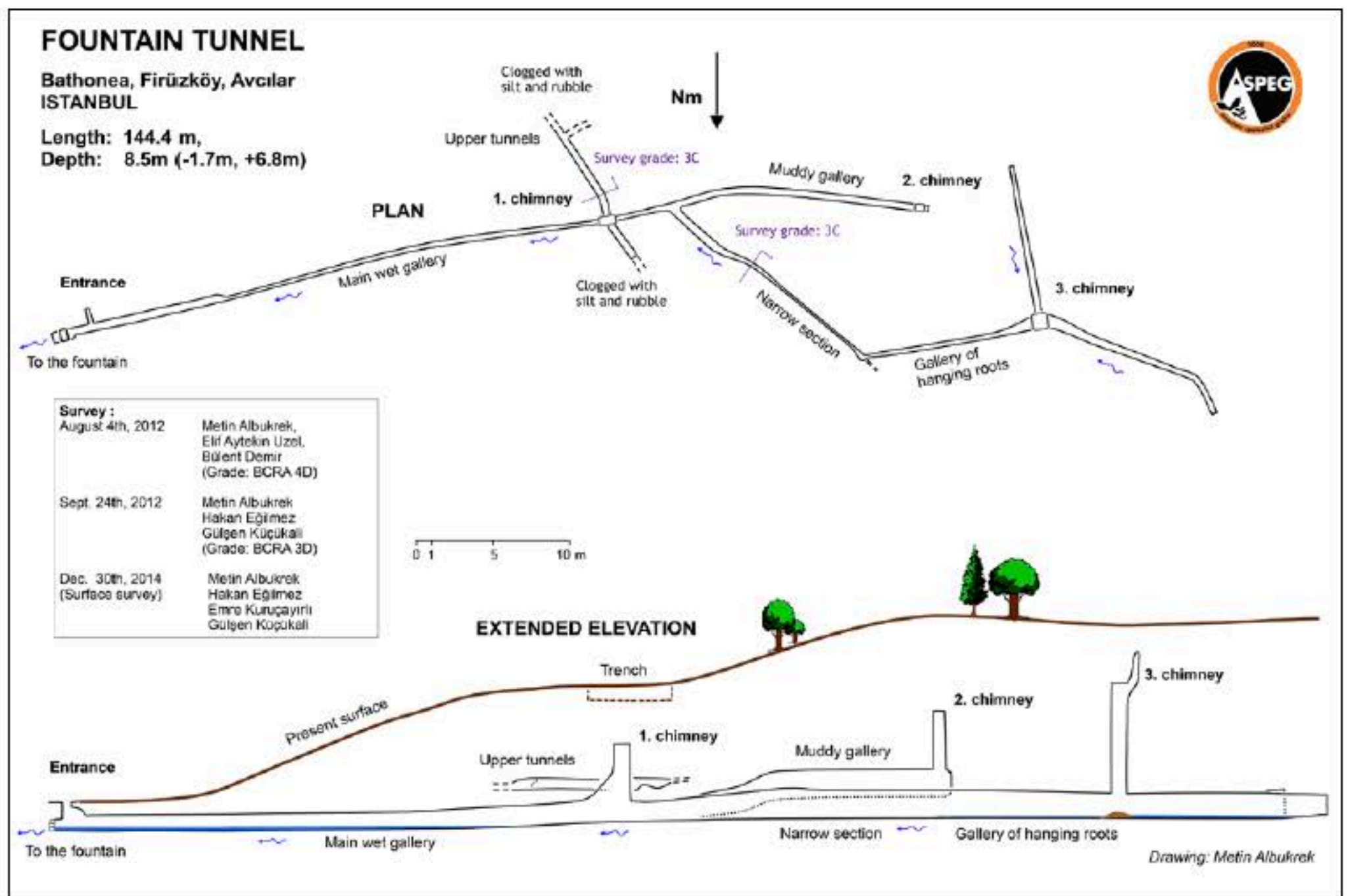
Fig. 4: plan of the Fountain Tunnel.
