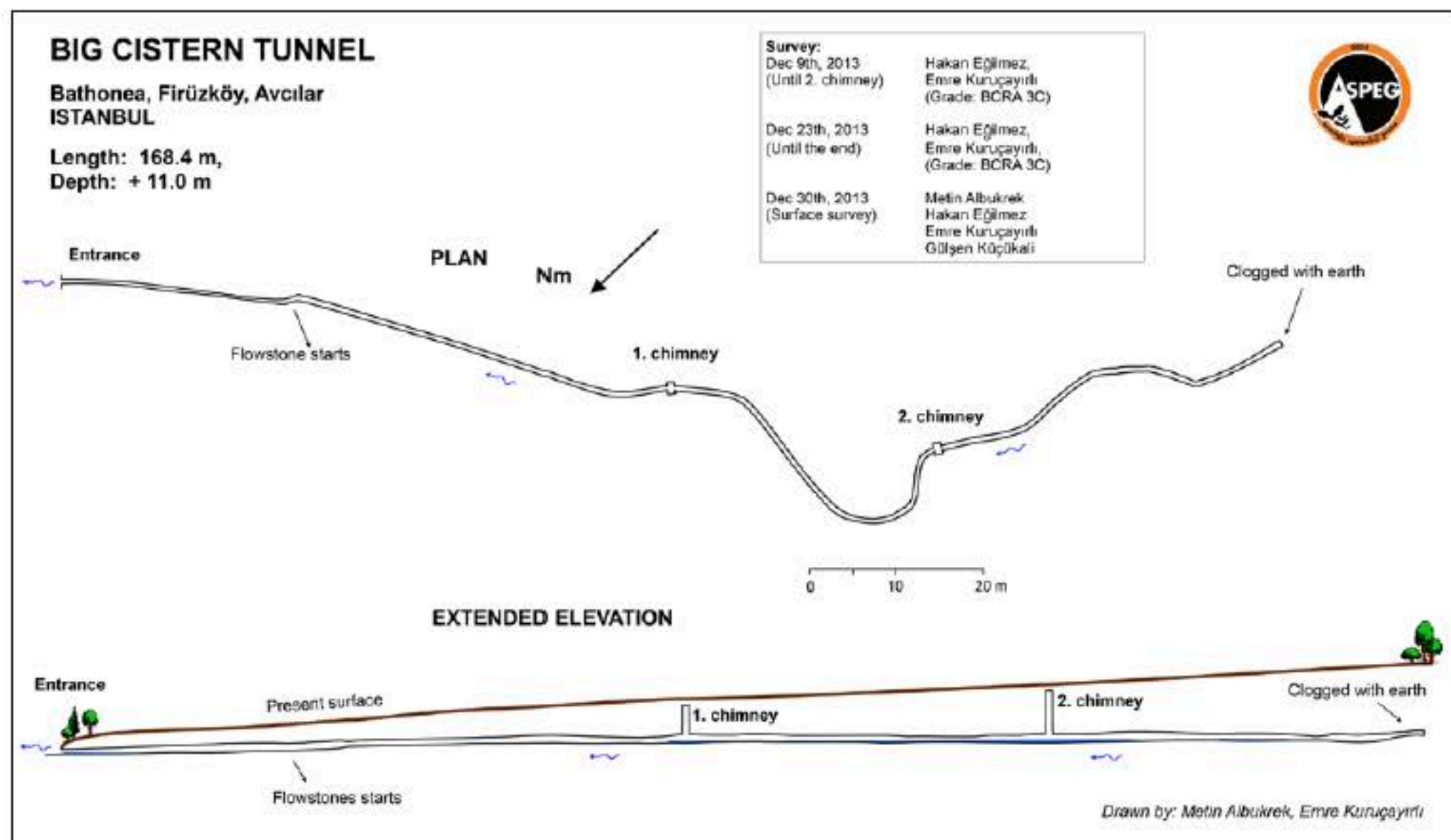
Fig. 11: plan of the Big Cistern Tunnel.
